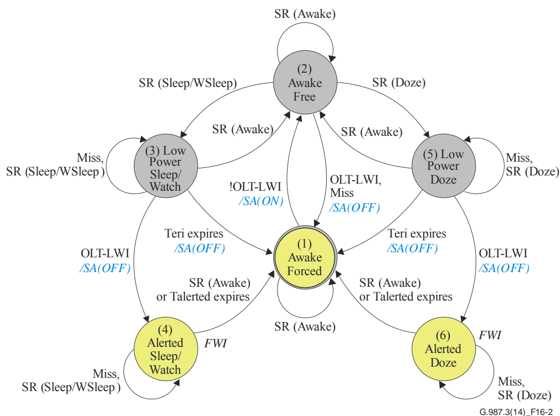
Figure 16-2 – OLT state transition diagram (initial state circled)
