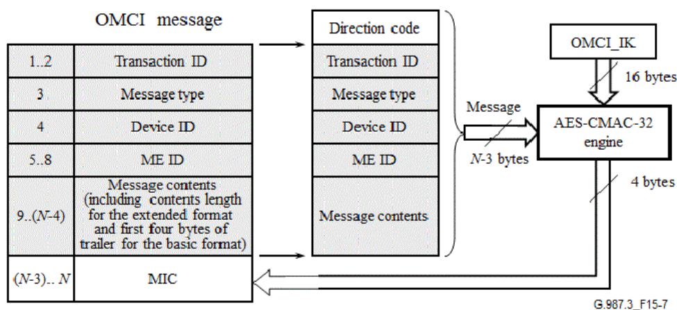
Figure 15-7 – OMCI integrity protection
