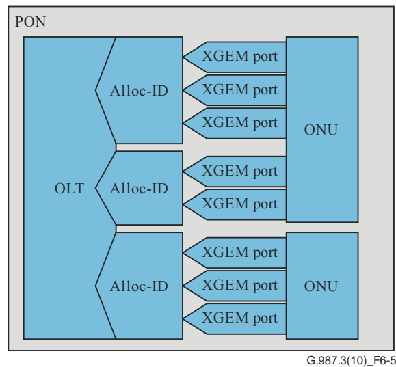
Figure 6-5 – Upstream multiplexing in XG-PON
