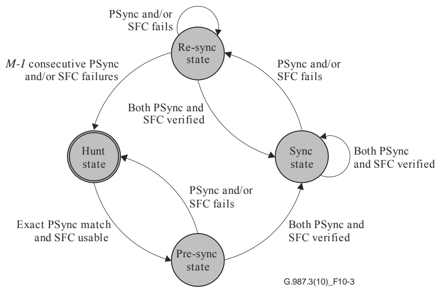
Figure 10-3 – Downstream ONU synchronization state machine
